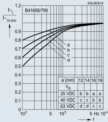
Frequency factor of permissible ripple current I_f versus frequency f
