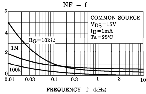
NOISE FIGURE NF (dB)
