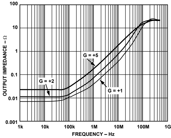
Figure 46. Output Enabled— Impedance vs. Frequency
