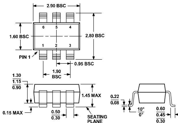
Figure 61. 6-Lead Plastic Surface-Mount Package [SOT-23] (RT-6)—Dimensions shown in millimeters
