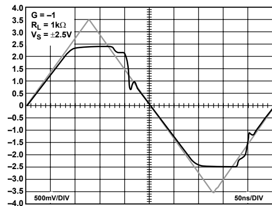
Figure 27. Output Overdrive Recovery
