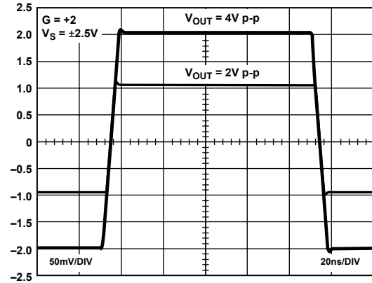
Figure 25. Large Signal Transient Response, G = +2
