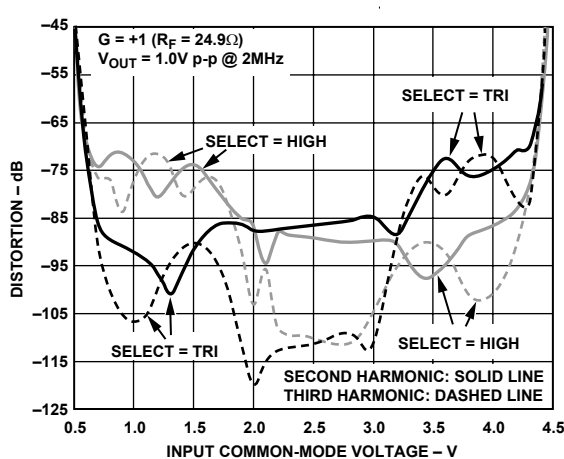
Figure 20. Harmonic Distortion vs. Input Common-Mode Voltage, V_S = +5V
