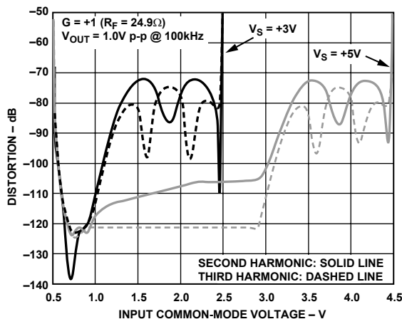
Figure 21. Harmonic Distortion vs. Input Common-Mode Voltage, SELECT = Tri-State or Open
