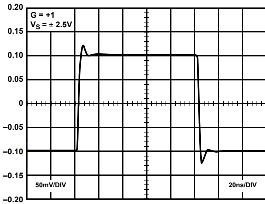
Figure 23. Small Signal Transient Response
