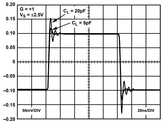
Figure 26. Small Signal Transient Response with Capacitive Load
