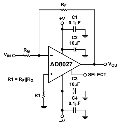
Figure 54. Wideband Inverting Gain Configuration
