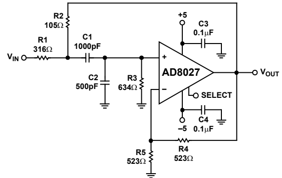
Figure 58. Band-Pass Filter Schematic
